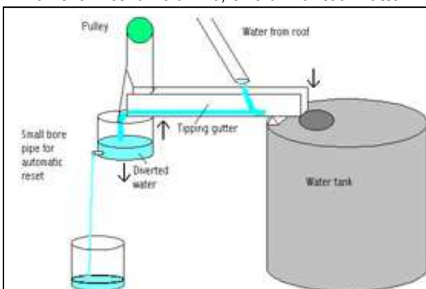
Figure 7a: Tipping gutter mechanism
